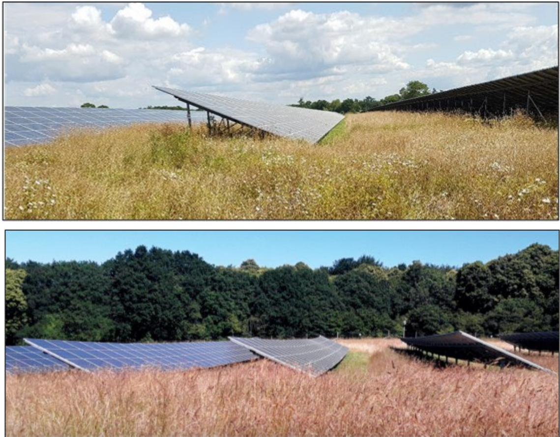
Figure 4.3: Sites where a “Shade Cut” has been employed during the growing season to prevent shading of panels, but allow flowering meadow elsewhere
